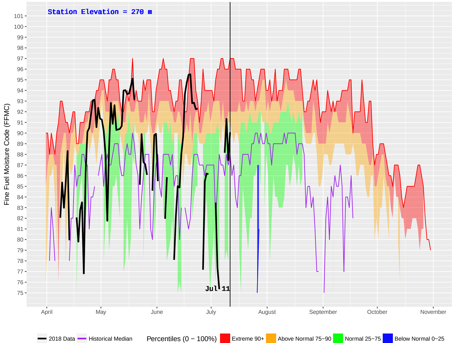
TALCHAKO (233) : Historical (1990–2016) and Current (2018) Noon Fine Fuel Moisture Code (FFMC)
